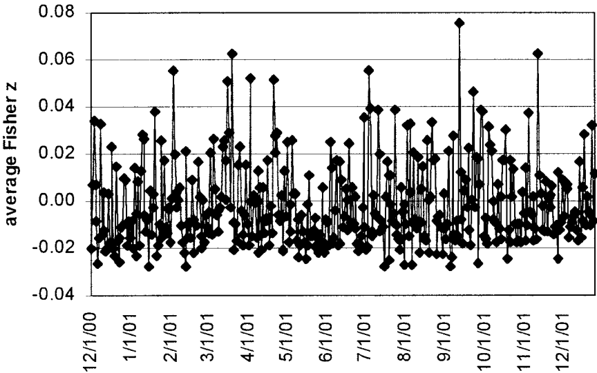
Fig. 4. Daily average RNG intercorrelations. The peak value is September 11, 2001.
