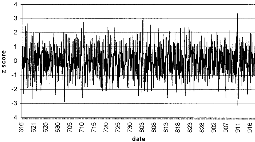
Fig. 2. z Scores associated with 6-hour sliding windows, as described in Steps 7 and 8 above, for RNG data collected between June 16, 2001 (noted as “616” on the x-axis) and September 20, 2001. This 3-month time-span was used to place the September 11 results into context.
